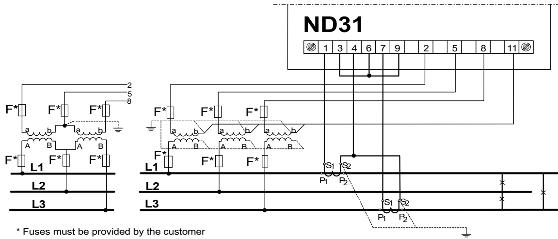
Fig 7. Connections of input signals in 3-phase 3-wire network
