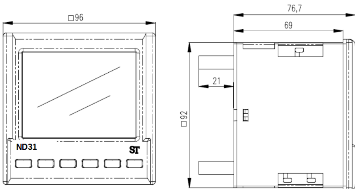
Fig. 3. Overall dimensions of the ND31 meter
