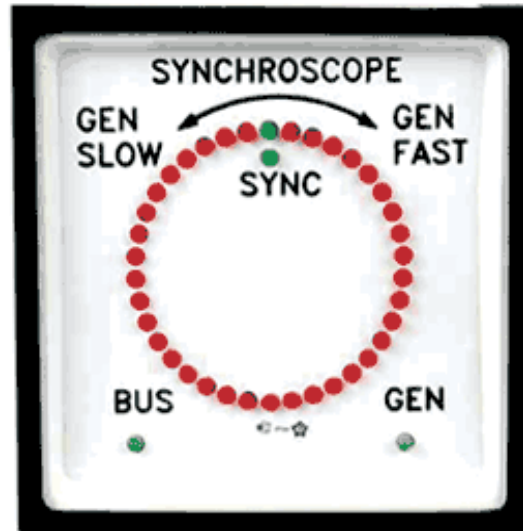
DIN LED Synchroscope Available in 96x96 mm and 144x144 mm DIN cutout sizes
