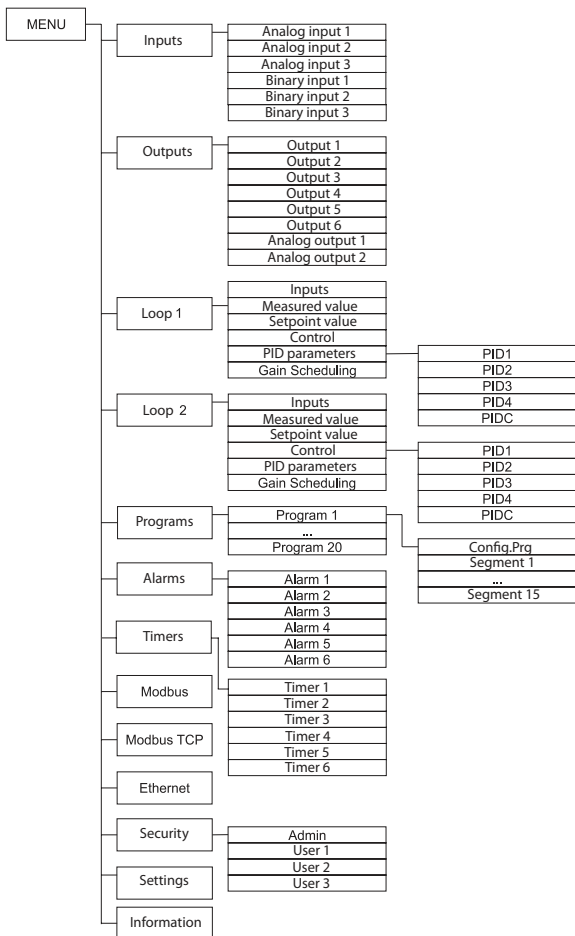
Fig. 14. Programming matrix
