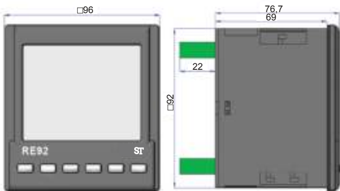
Fig. 2. Controller dimensions.
