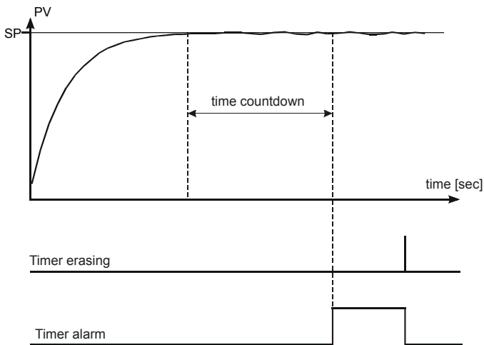
Fig.23. Principle of timer operation
